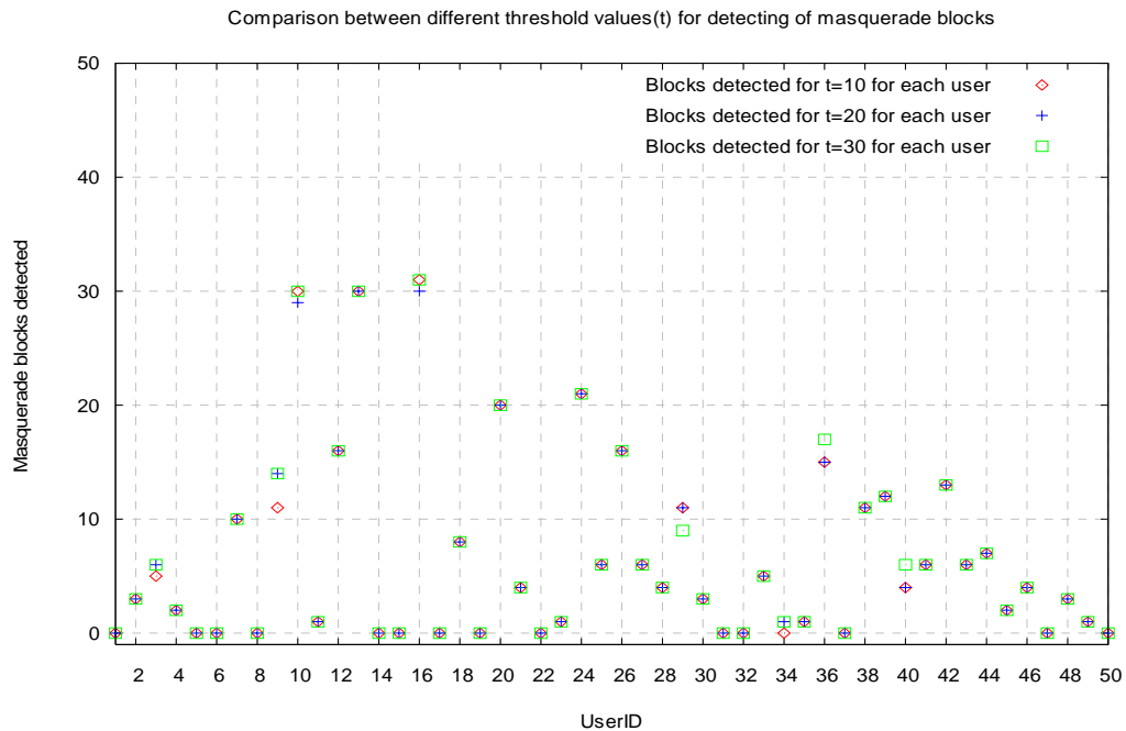
Figure 5.3 Comparison of detection of masquerades in each block for different (t)
