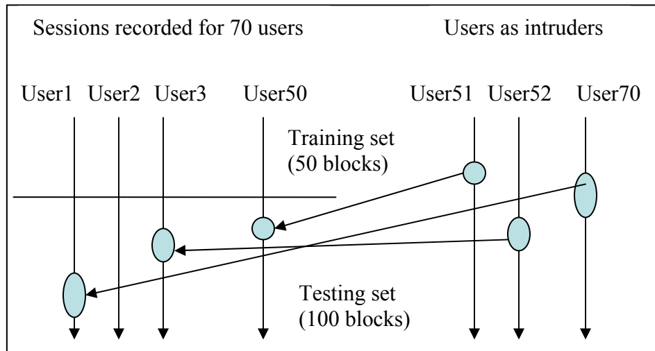
Figure 4.1. Splicing of sessions
