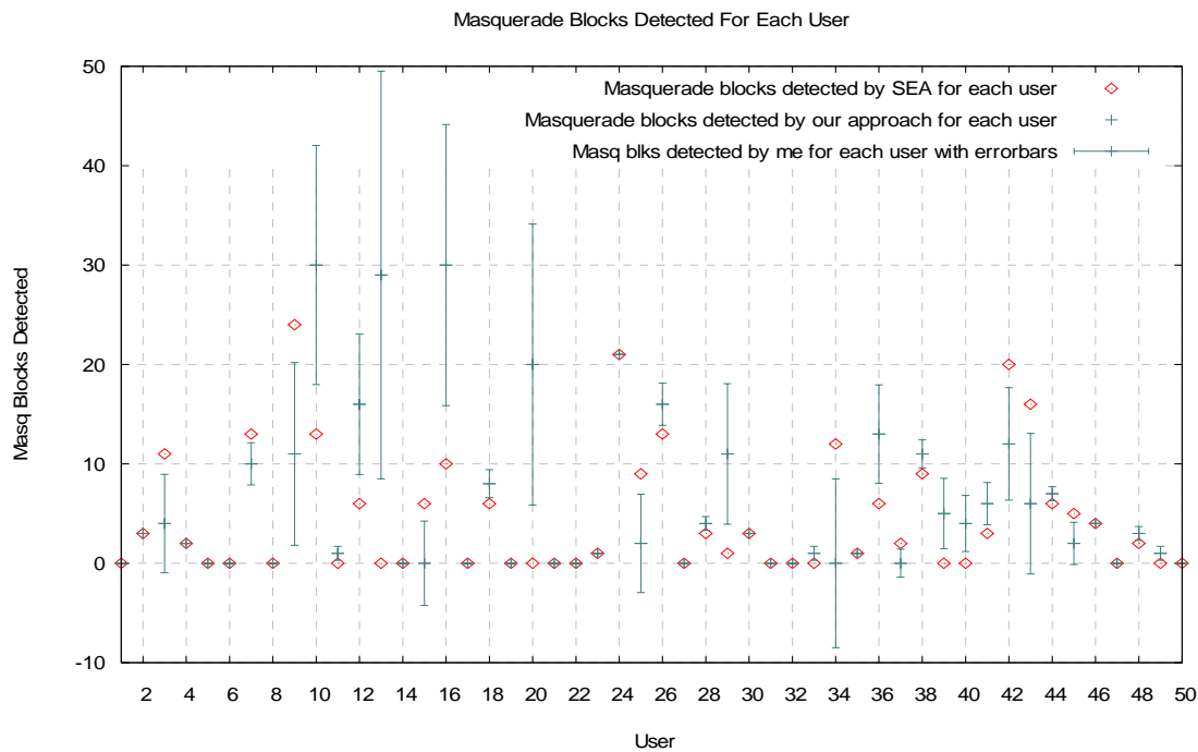
Figure 5.4. Detection of masquerade blocks with error analysis
