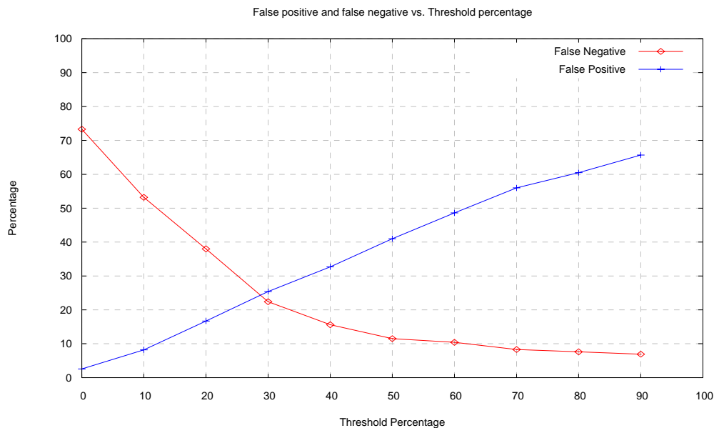
Figure 5.2 False positive and false negative vs. threshold percentage.
