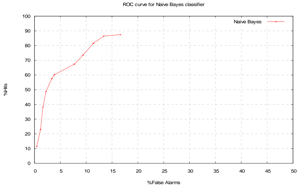
Figure 5.1. Relative operating characteristic (ROC) curve for the naïve Bayes classifier
