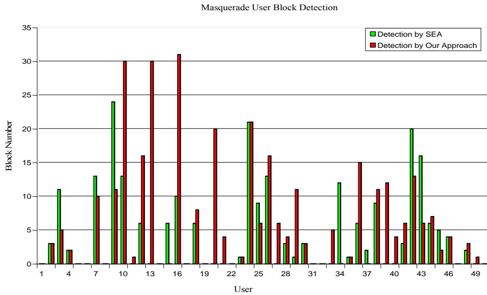
Figure 5.5. Comparisons of the masquerade block and user detection by our approach and the SEA approach.
