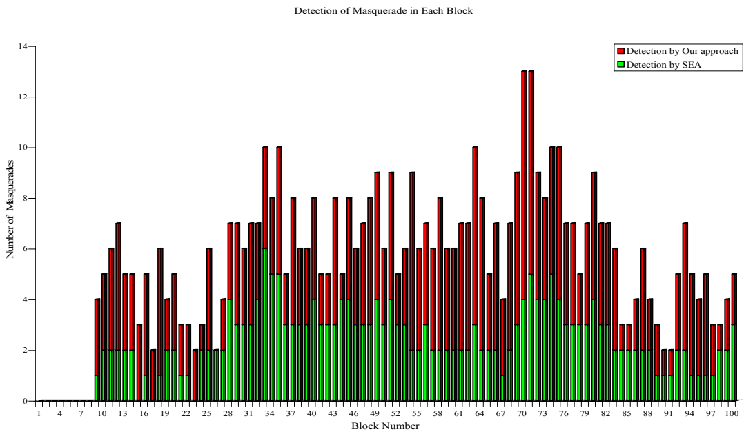
Figure 5.6. Comparison of the number of masquerades detected in each block by our approach and the SEA approach
