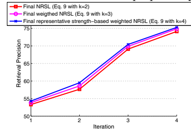
Fig. 4: Comparisons of three NRSL systems incorporating N and expanding P
