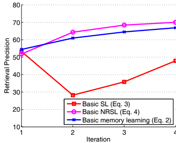
Fig. 2: Comparisons of basic memory learning and two SL systems without incorporating N and expanding P
