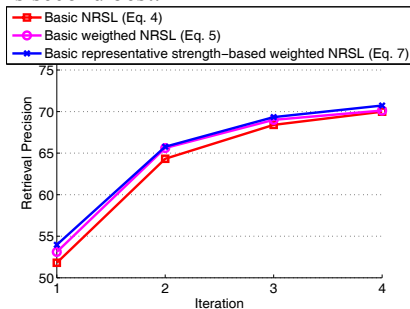
Fig. 3: Comparisons of three NRSL systems without incorporating N and expanding P
