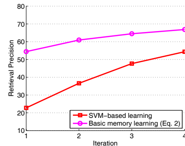
Fig. 1: Accuracy of SVM-based and basic memory learning
